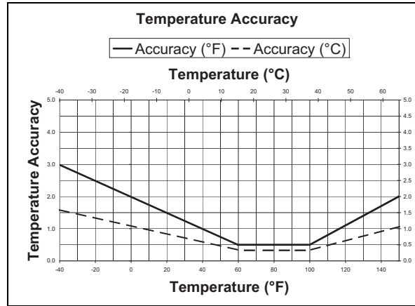
Figure 1. Temperature Accuracy
